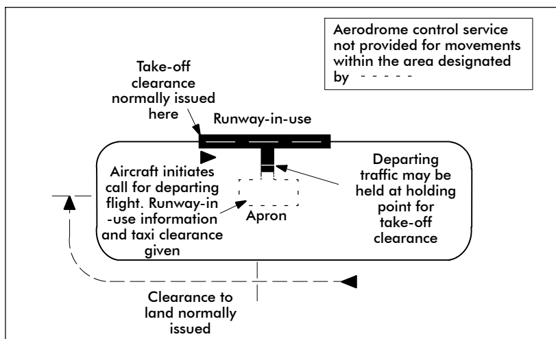
Figure AD 1.6 - 1 Postions for Clearance at Controlled Aerodromes
